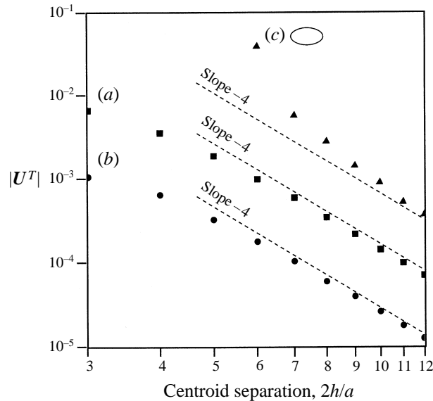
FIGURE 4. Drop velocity of perfect dielectric drops as a function of centroid (centre-to-centre) position. Dashed lines show the expected h^{-4} dependence of the electrically-driven centre-of-mass velocities. (a) \bar{\epsilon}/\epsilon = 5 , \lambda = 1 , \mathcal{C}_e = 0.1 , 1% maximum deformation; (b) \bar{\epsilon}/\epsilon = 0.4 , \lambda = 1 , \mathcal{C}_e = 1 , 5% maximum deformation; (c) \bar{\epsilon}/\epsilon = 8 , \lambda = 1 , \mathcal{C}_e = 1 , 57% maximum deformation.
